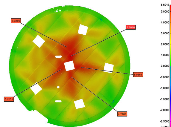
Tank Bottom Elevation Colour Plot (Inches)
