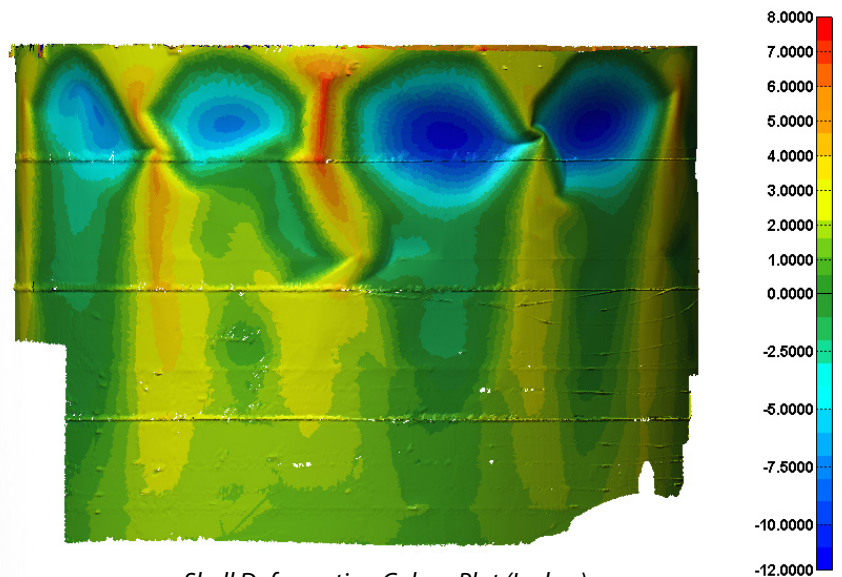
Shell Deformation Colour Plot (Inches)
