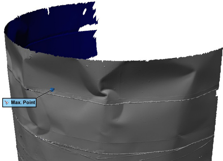
3D Laser Measurement of Tank Shell Deformations
